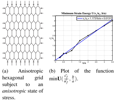
Figure 5: Derivation of the relationship \min U_a(\frac{\vec{v}_f^*}{u_f}, \frac{b}{a}) for an anisotropic hex-grid subject to an anisotropic state of stress.
