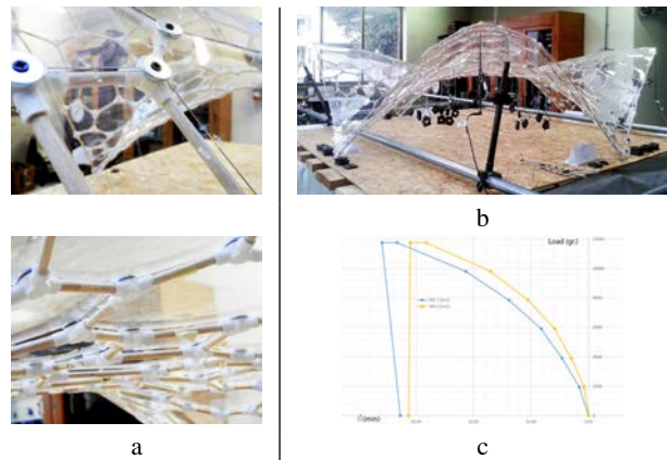
Figure 17: a. Some particular of the physical replica ; b. Setup for load tests over the fabricated model; c. displacement / external load plot.
